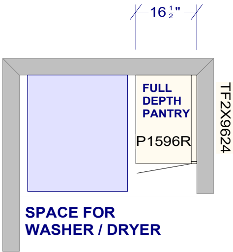
LAUNDRY ROOM
