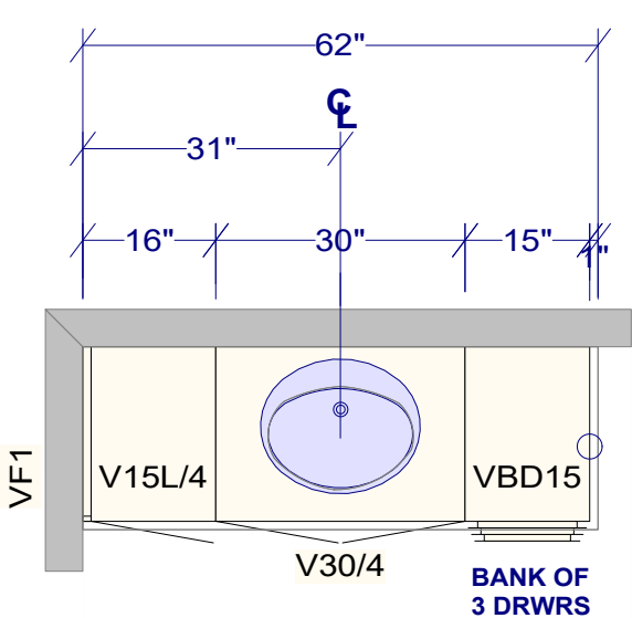
MAIN BATH
