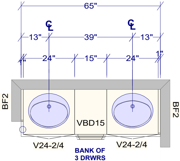
PRIMARY ENSUITE
