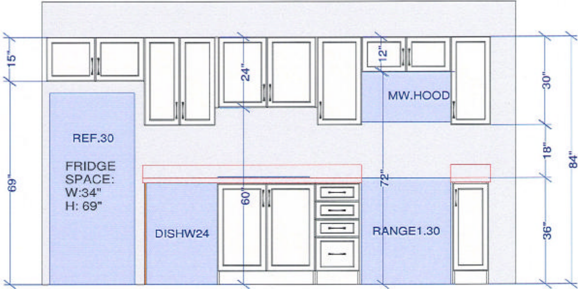
FRIDGE / SINK/ RANGE WALL ELEVATION
