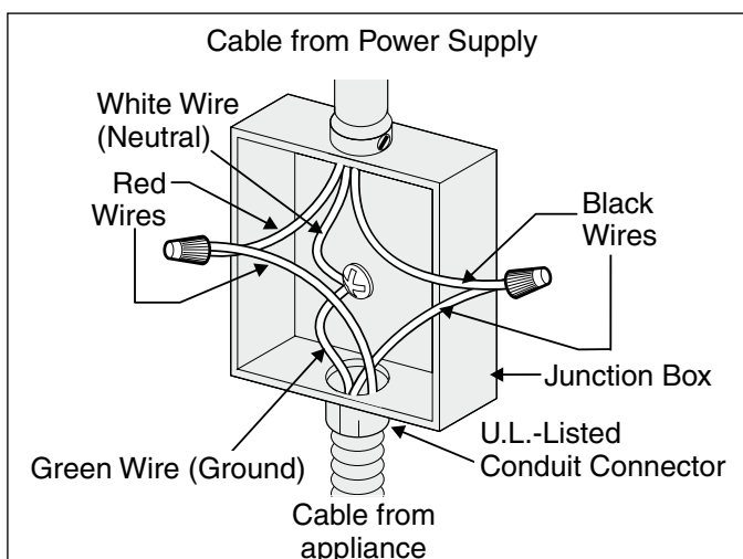
Figure 3 - 3-WIRE GROUNDED JUNCTION BOX
