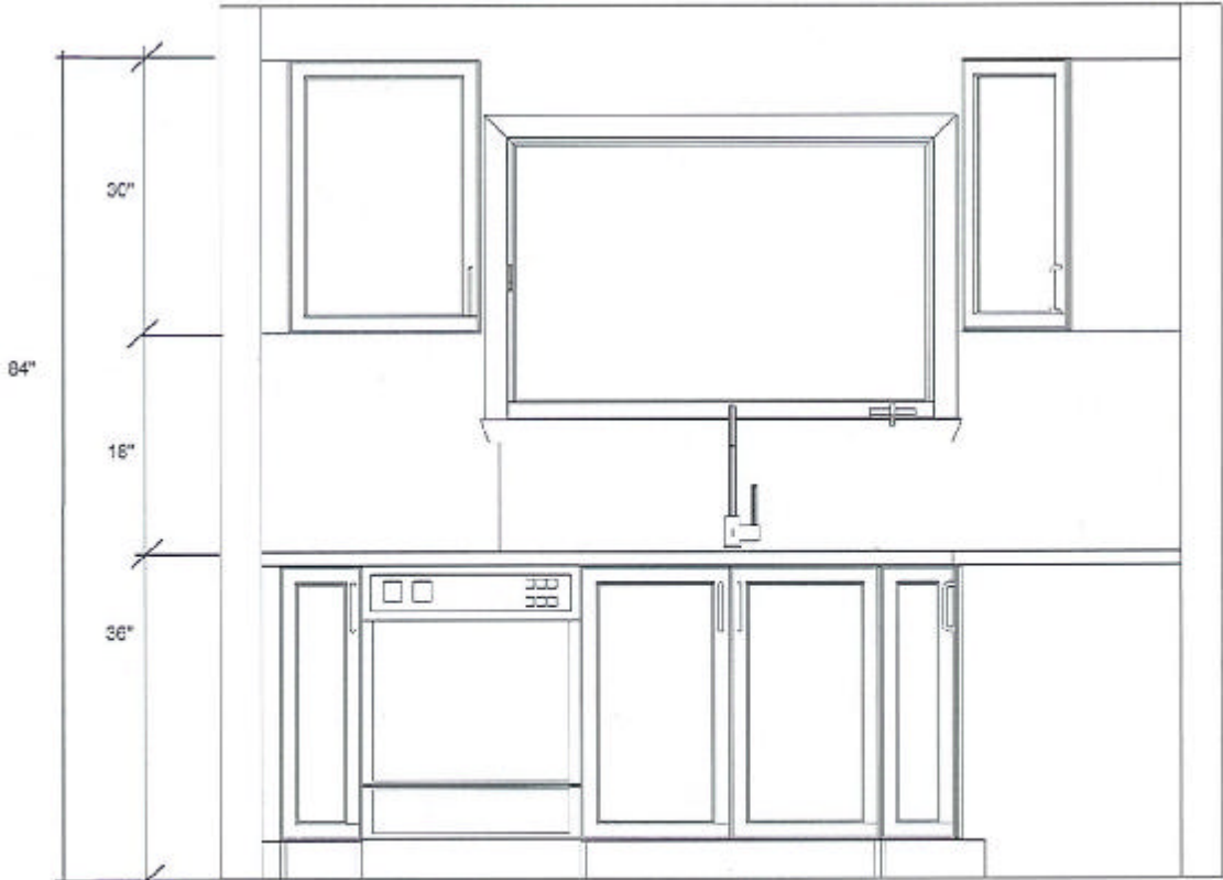
BASEMENT KITCHEN - SINK WALL ELEVATION 35-32 MIRAPOSA
