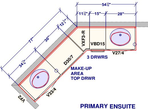
PRIMARY ENSUITE
