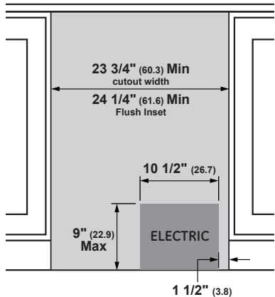
INSTALLATION CUTOUT FRONT VIEW
