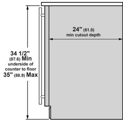
INSTALLATION CUTOUT SIDE VIEW
