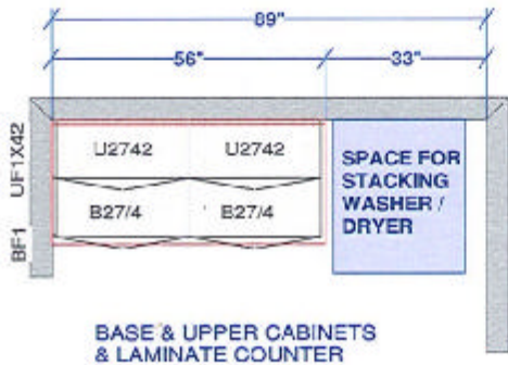
LAUNDRY ROOM
