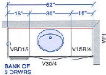
MAIN BATH
