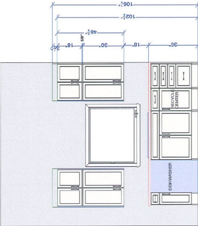
SINK WALL ELEVATION
