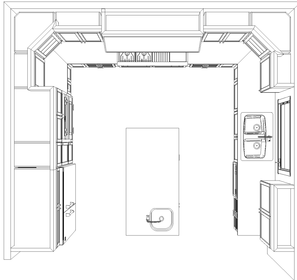
KITCHEN - TOP VIEW
