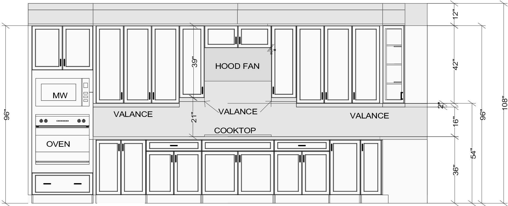
OVEN / COOKTOP WALL ELEVATION
