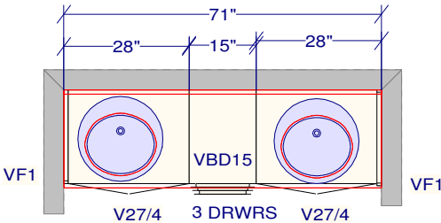
ALTERNATE MAIN SHARED BATH BDRM 3 & 4
