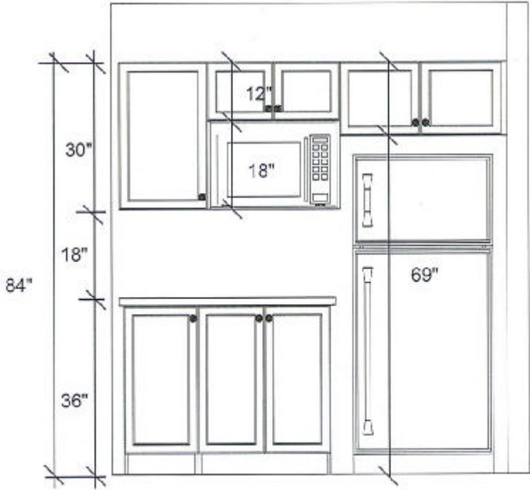
DCR PHOENIX - 517 RUTHERFORD STD FRIDGE WALL ELEVATION
