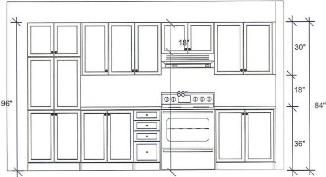
DCR PHOENIX 517 RUTHERFORD STD STOVE WALL ELEVATION
