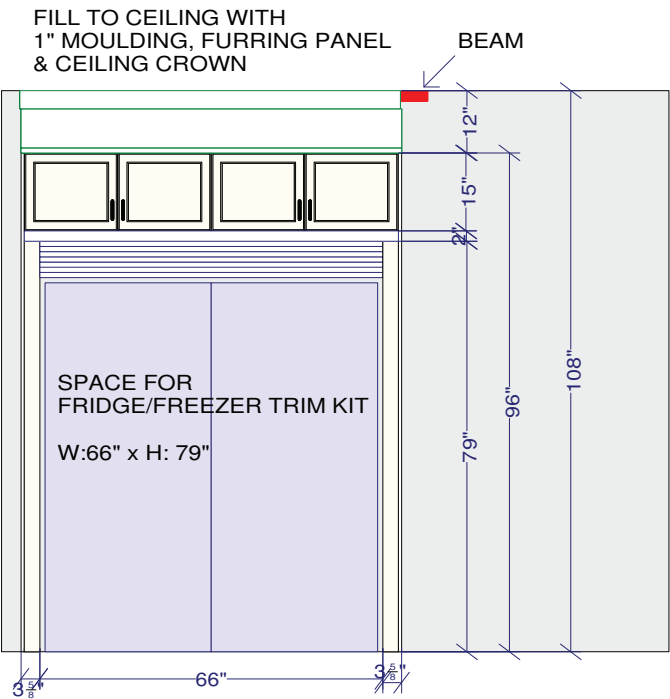
FRIDGE/FREEZER WALL ELEVATION
