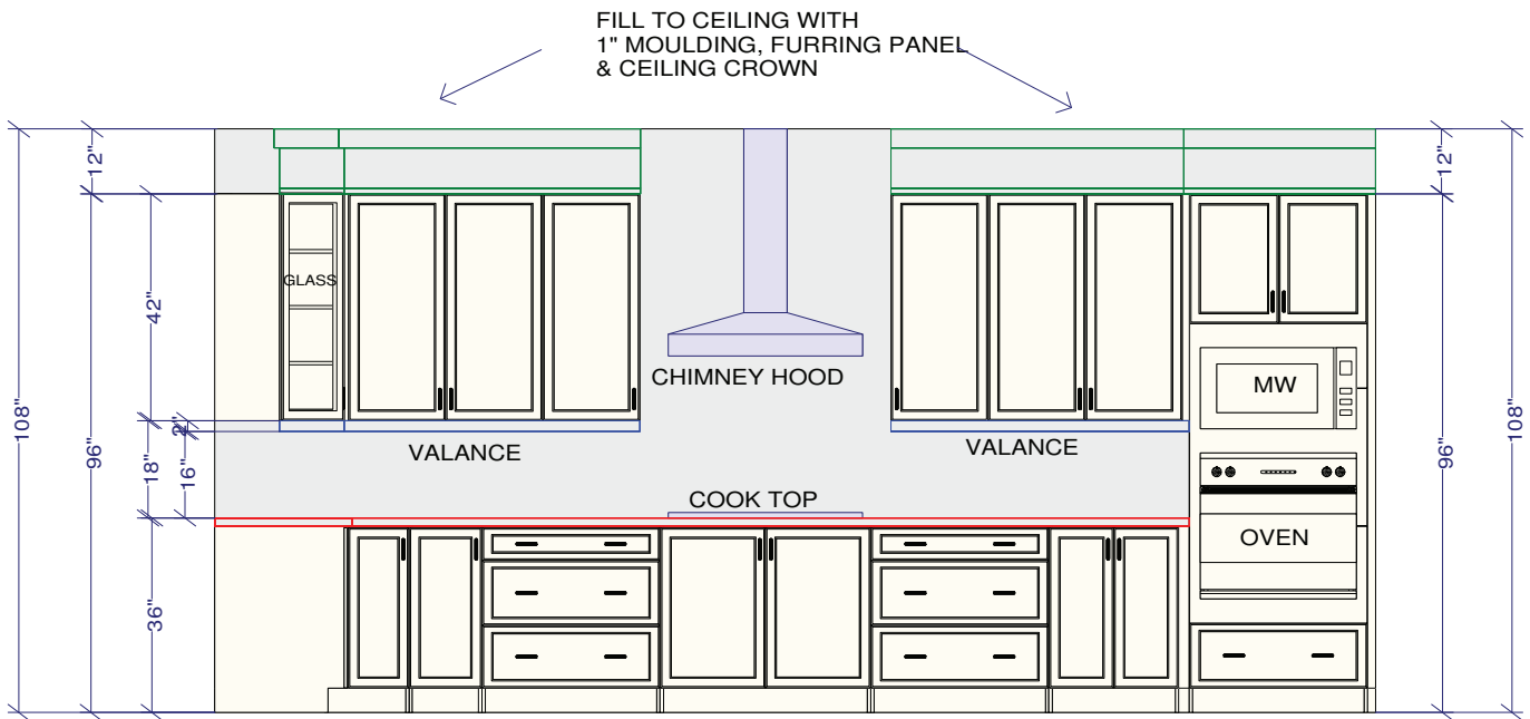
COOKTOP WALL ELEVATION
