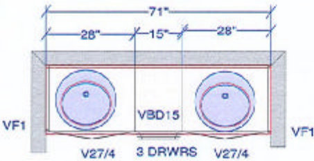
ALTERNATE MAIN SHARED BATH BDRM 3 & 4
