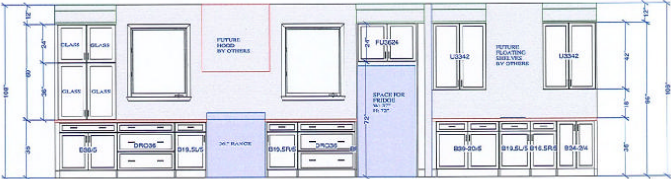
RANGE / FRIDGE WALL ELEVATION
