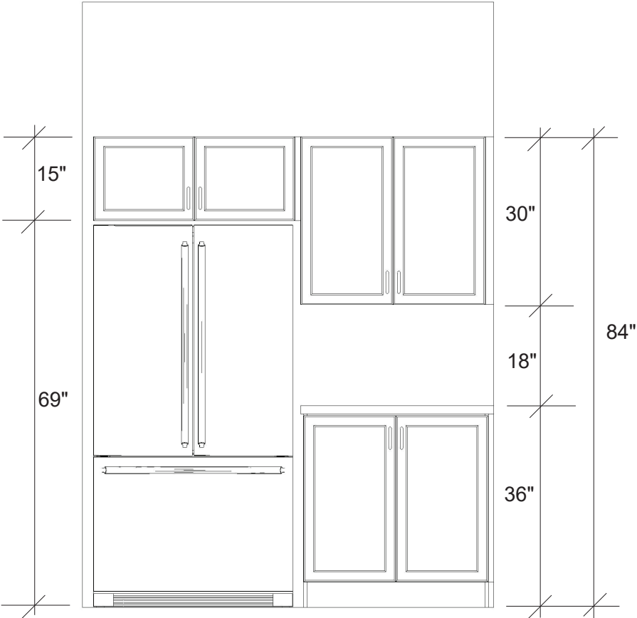
FRIDGE ELEVATION
