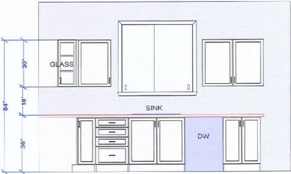
SINK WALL ELEVATION
