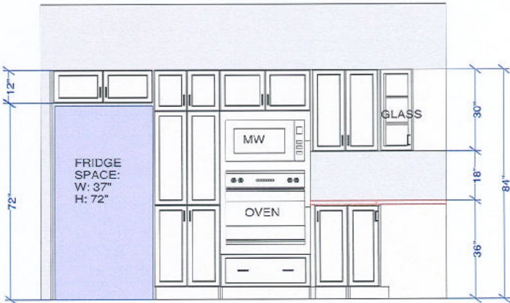
FRIDGE / OVEN WALL ELEVATION
