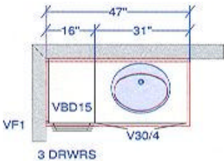
IN LAW - ENSUITE
