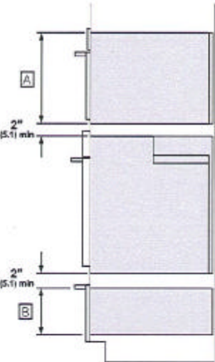
STANDARD INSTALLATION SIDE VIEW
