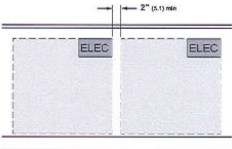
SIDE-BY-SIDE INSTALLATION FRONT VIEW OF CUTOUTS
