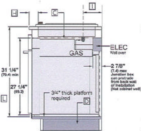
STANDARD INSTALLATION SIDE VIEW
