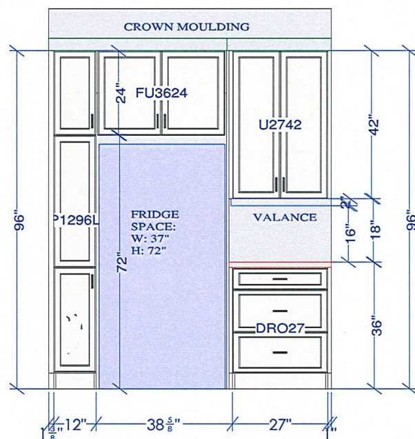
FRIDGE WALL ELEVATION
