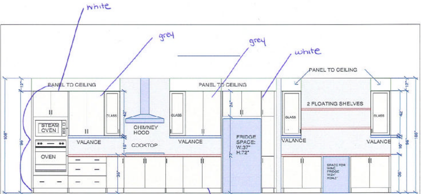
OVEN / COOKTOP / FRIDGE WALL ELEVATION
