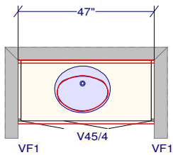
POWDER ROOM
