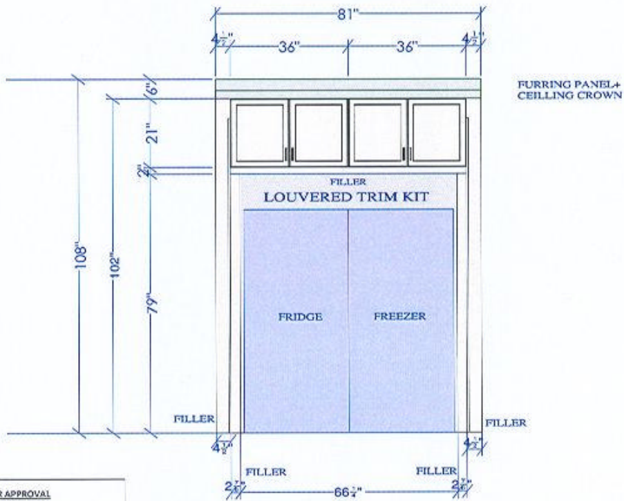
FRIDGE/FREEZER ELEVATION
