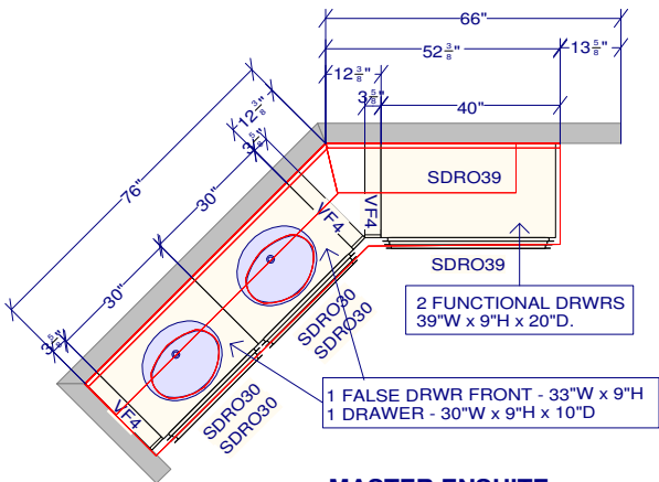
MASTER ENSUITE FLOATING VANITY @ 12.25" A.F.F.
