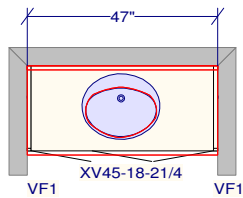
POWDER ROOM FLOATING VANITY @ 12.25" A.F.F.
