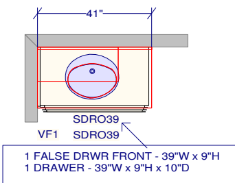
IN LAW - ENSUITE FLOATING VANITY @ 12.25" A.F.F.
