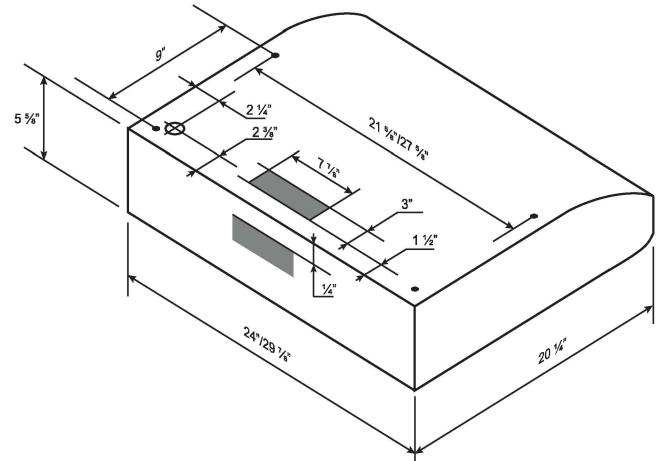
ISOMETRIC
