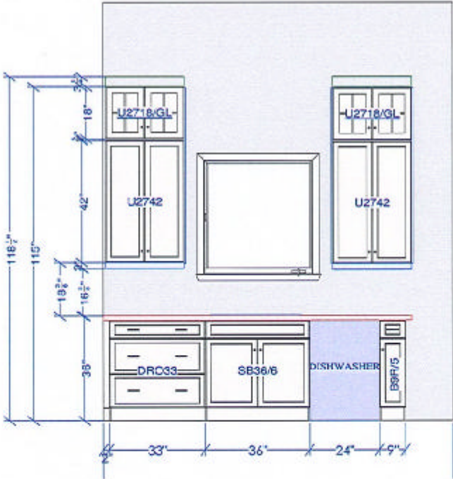
SINK WALL ELEVATION
