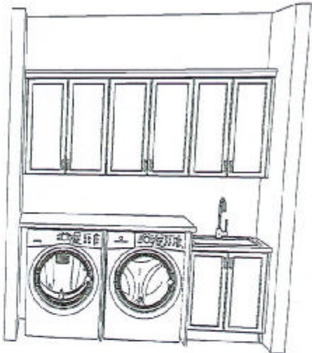
LAUNDRY
