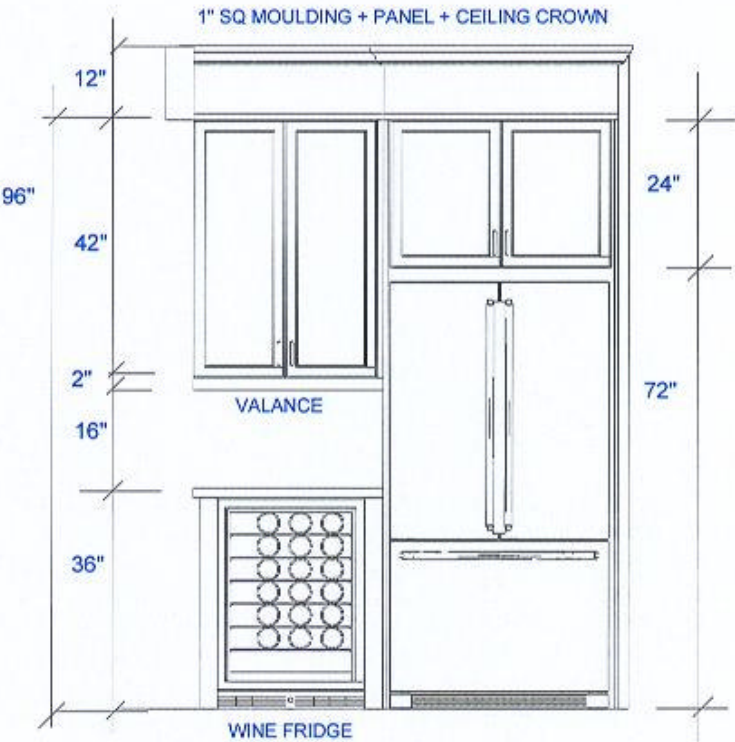
FRIDGE WALL ELEVATION
