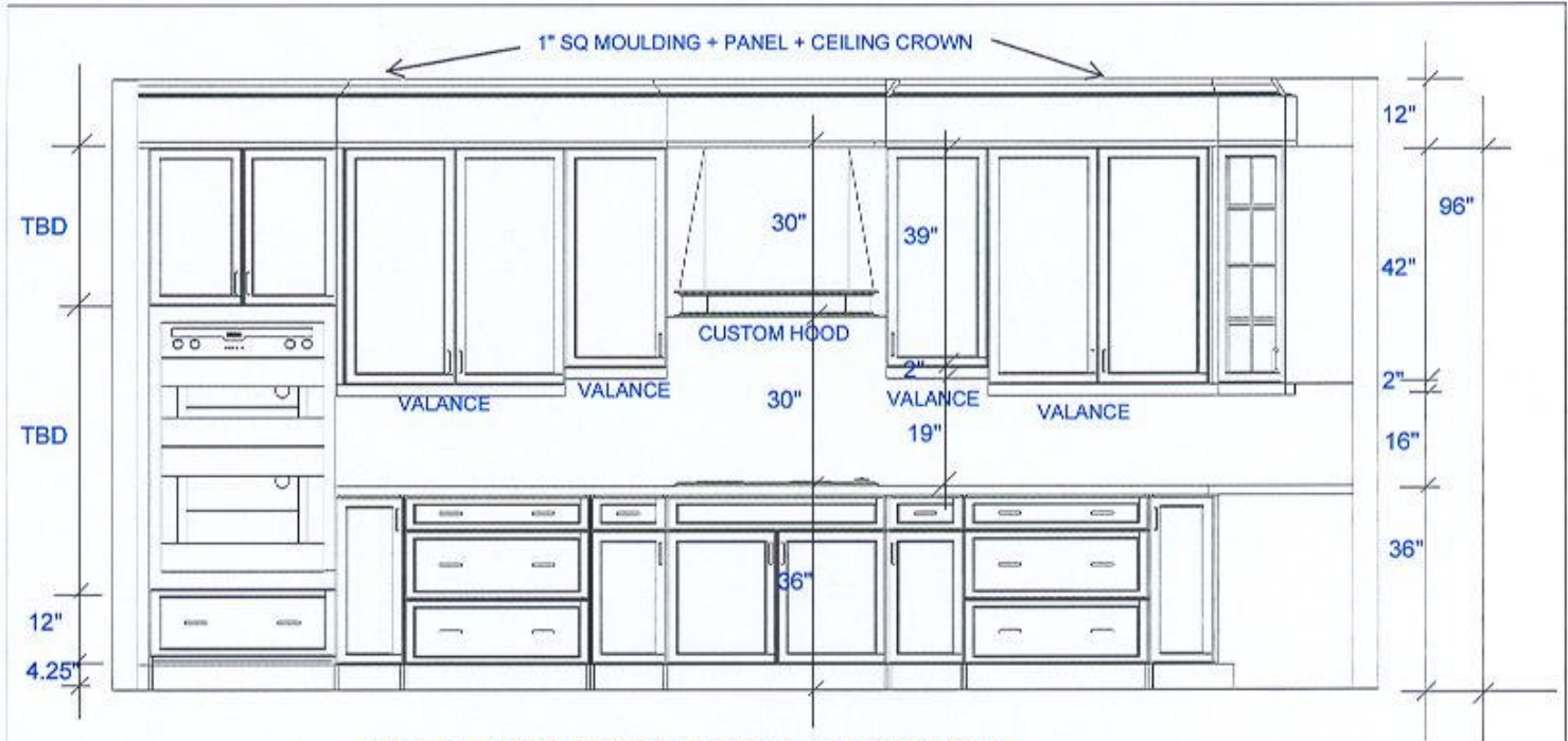
OVEN / COOK TOP WALL ELEVATION
