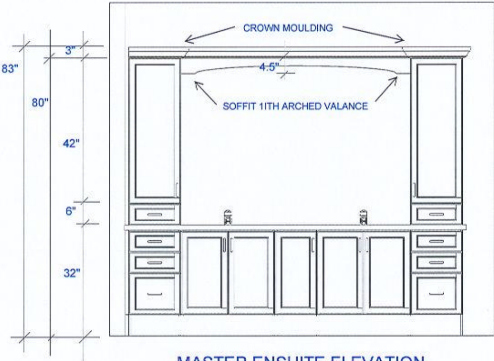
MASTER ENSUITE ELEVATION
