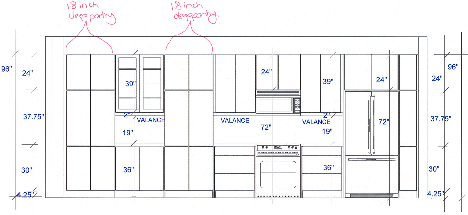
EATING AREA ELEVATION
