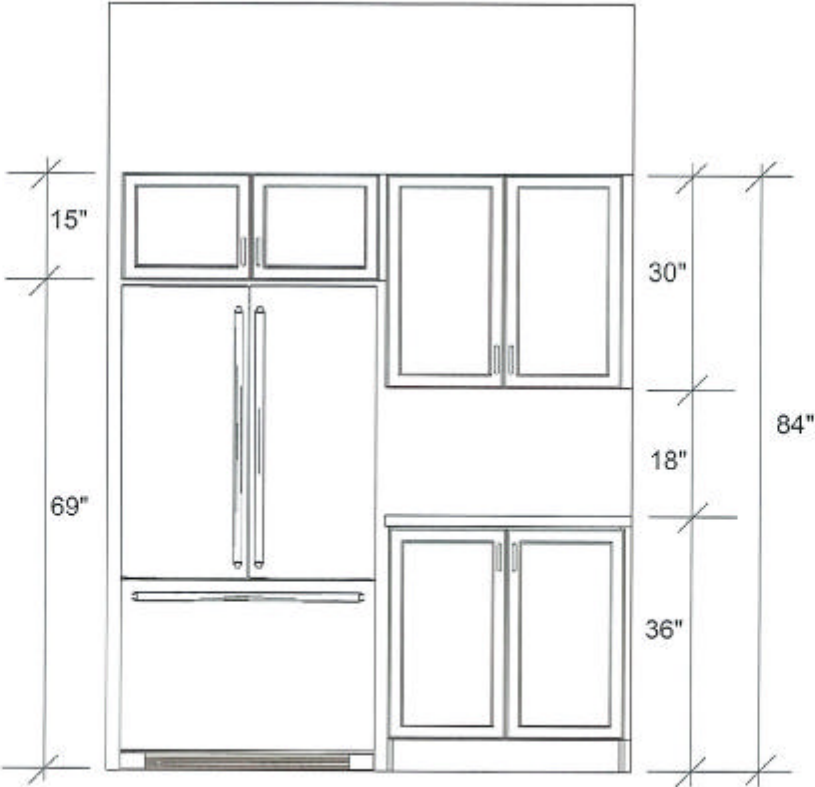
FRIDGE ELEVATION
