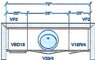
MAIN BATH
