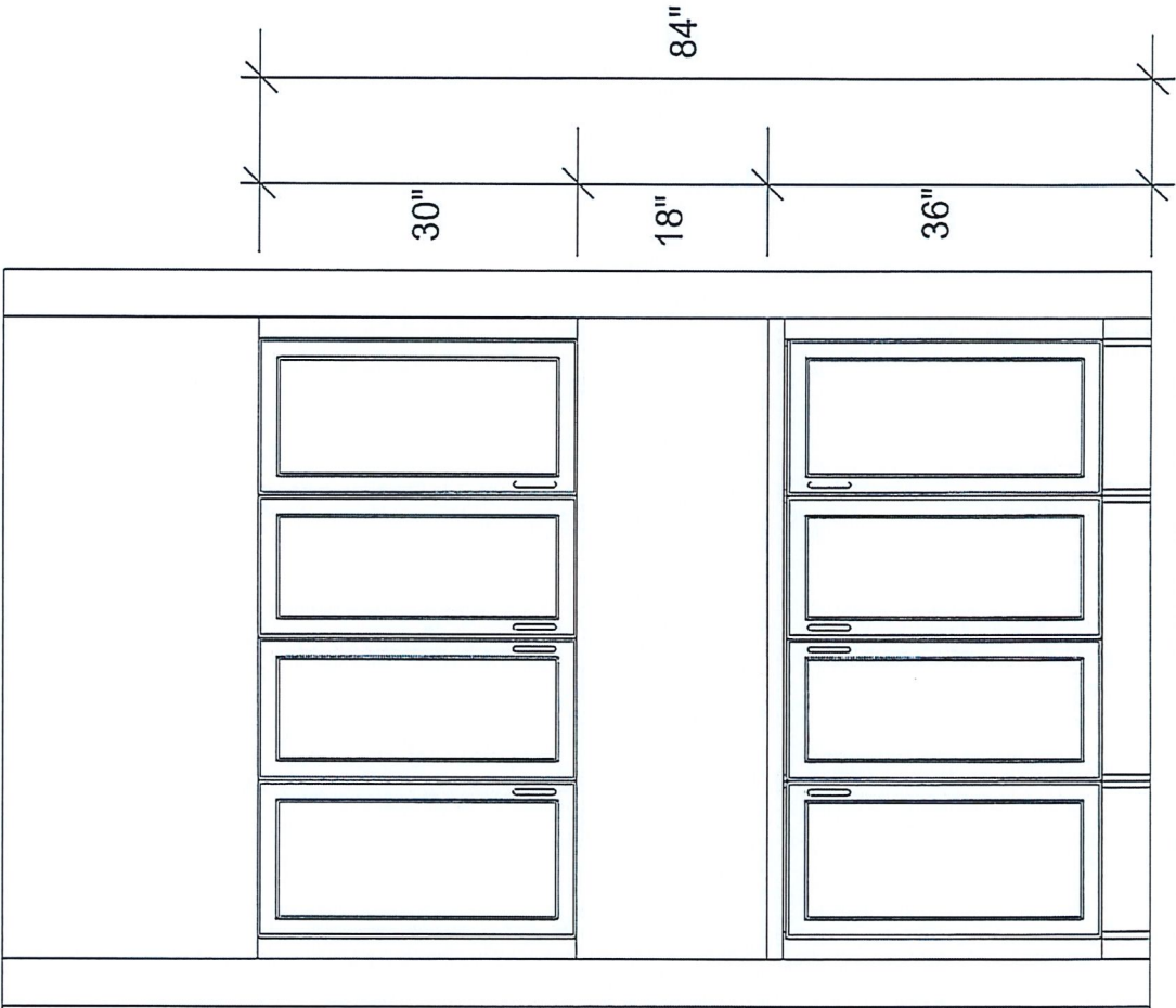
BUTLER'S PANTRY ELEVATION
