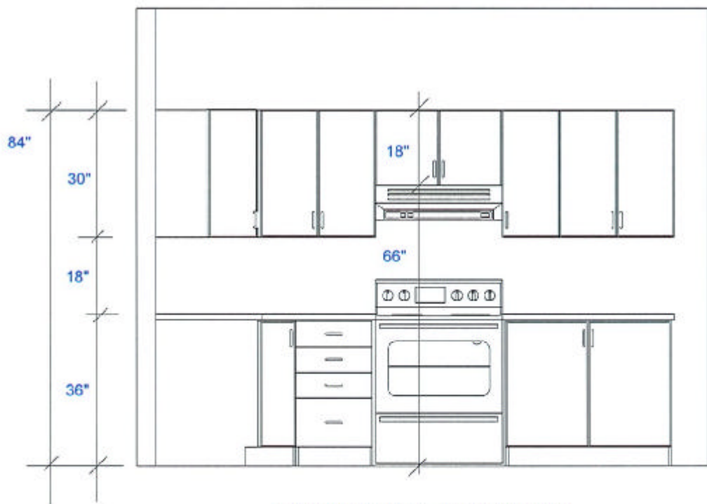
RANGE WALL ELEVATION
