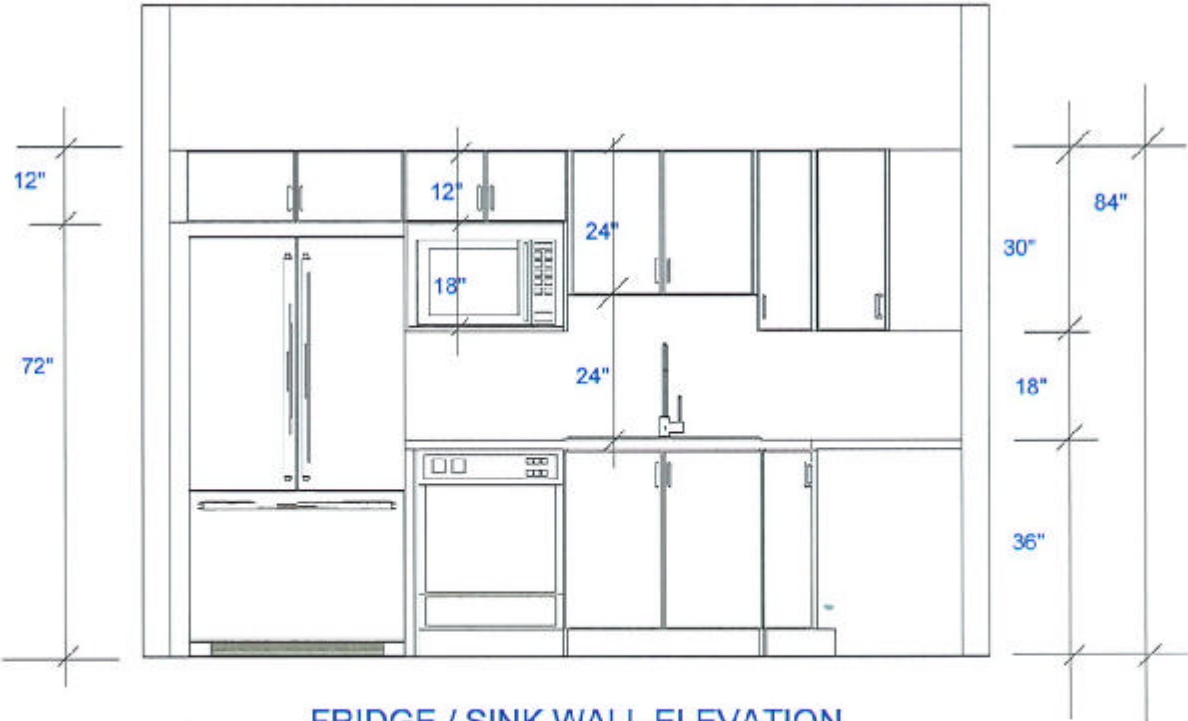
FRIDGE / SINK WALL ELEVATION
