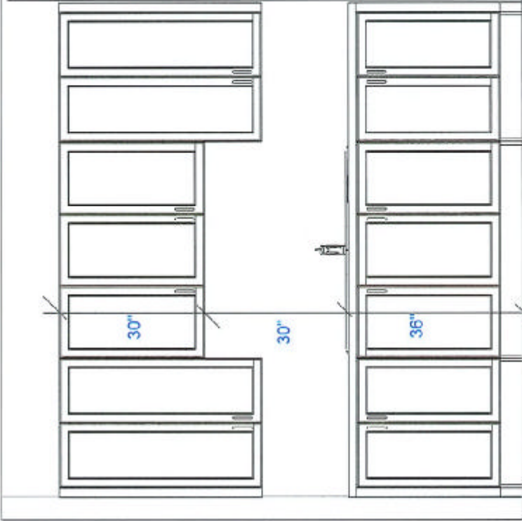
BUTLER'S PANTRY ELEVATION
