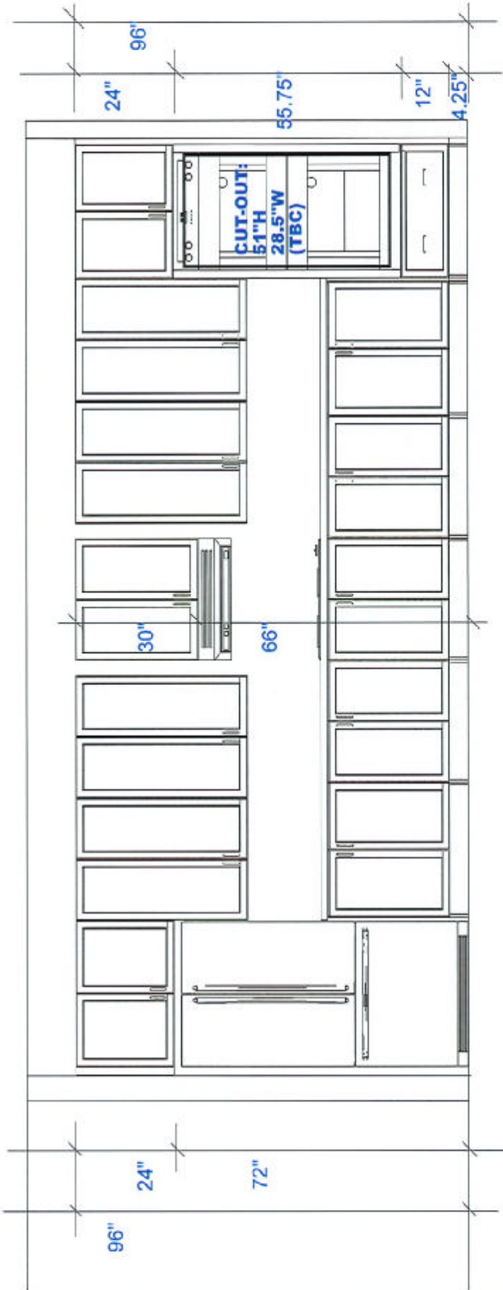
FRIDGE / COOKTOP / OVEN WALL ELEVATION
