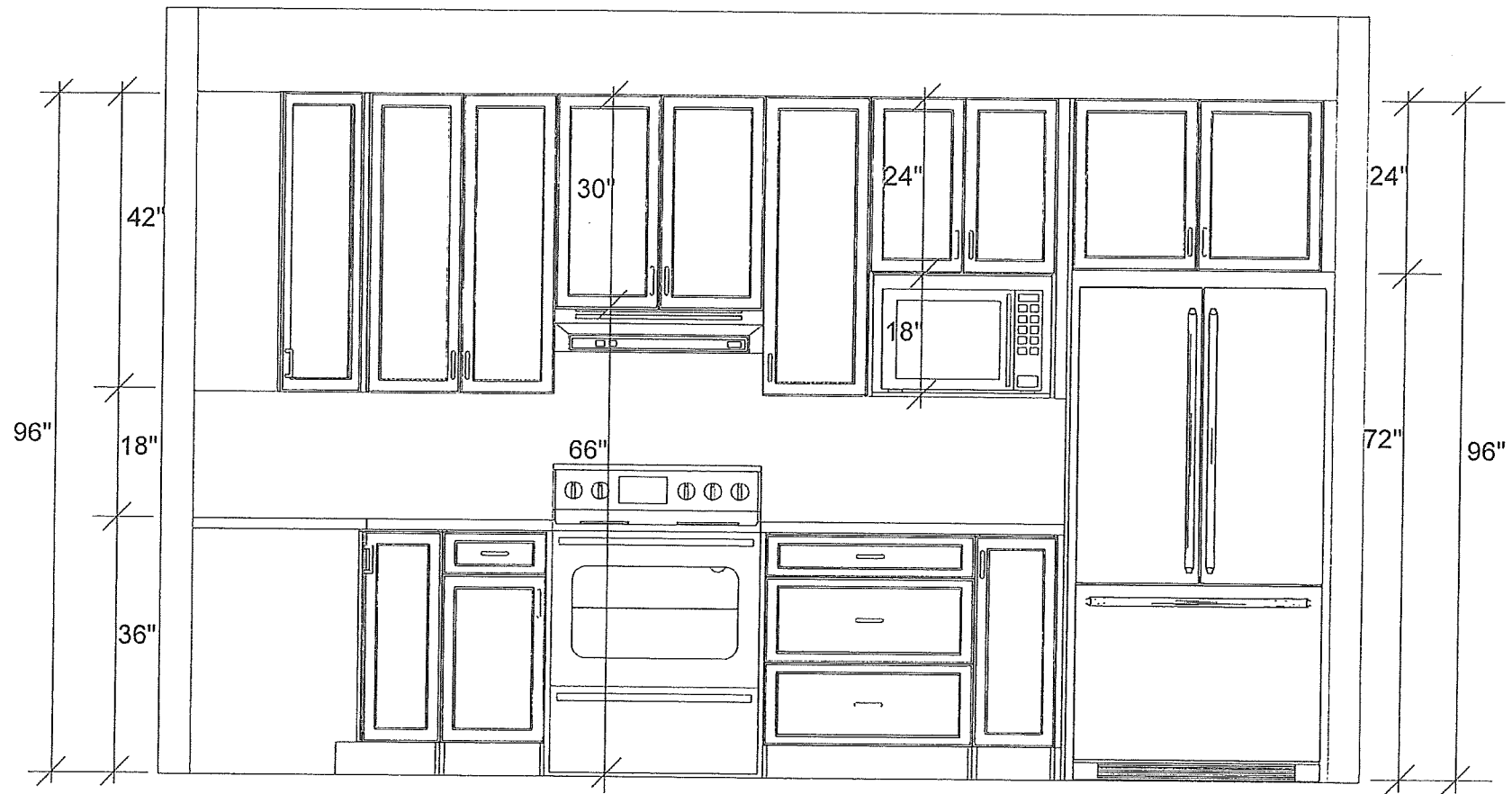
STOVE / FRIDGE WALL ELEVATION
