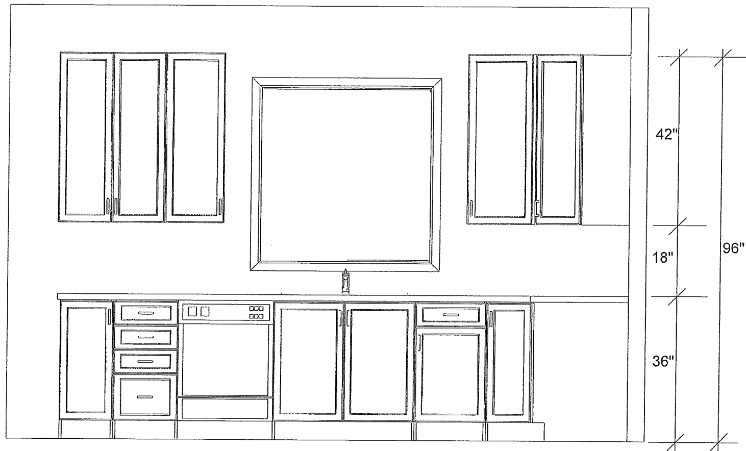
SINK WALL ELEVATION
