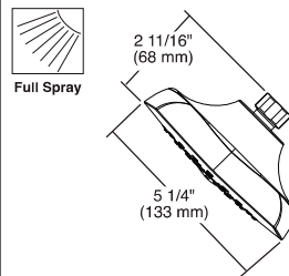
RP64859 Touch-Clean Raincan Shower Head 1.75 GPM
