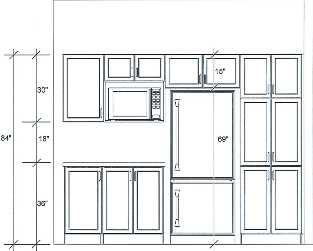
FRIDGE WALL ELEVATION
