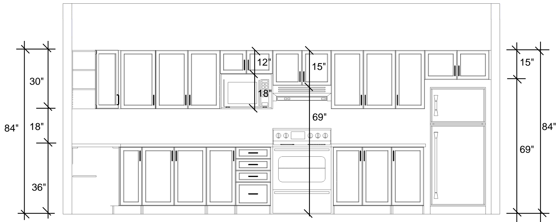
STOVE & FRIDGE WALL ELEVATION 509 ANNAPOLIS
