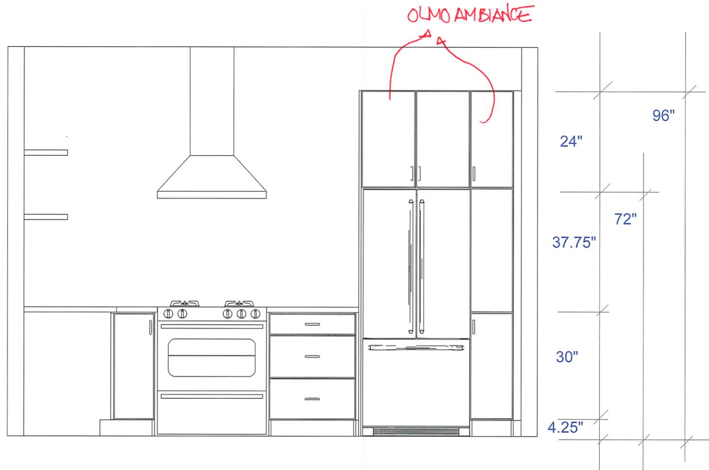
RANGE/ FRIDGE WALL ELEVATION
