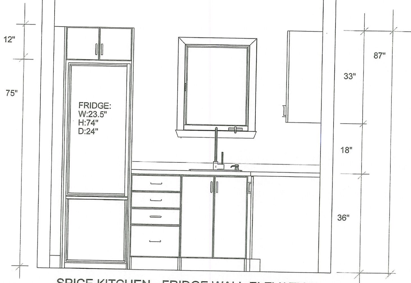
SPICE KITCHEN - FRIDGE WALL ELEVATION
