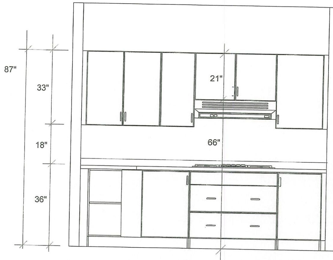
SPICE KITCHEN - COOKTOP WALL ELEVATION
