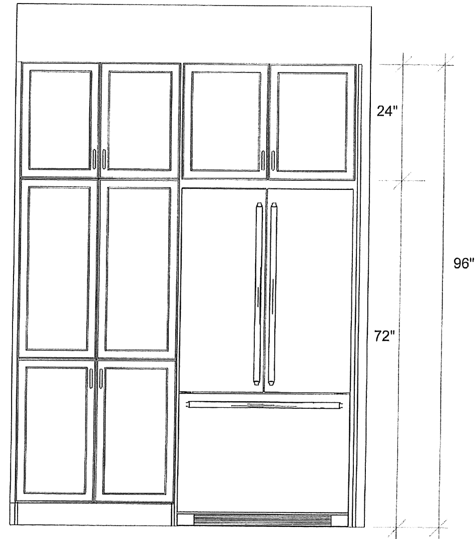
FRIDGE WALL ELEVATION
