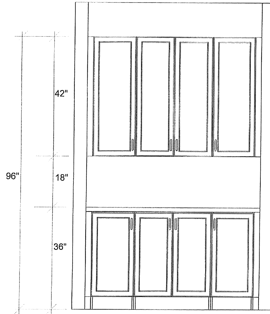
BUTLER'S PANTRY ELEVATION
