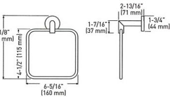
TOWEL RING
