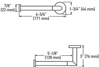
PAPER HOLDER
