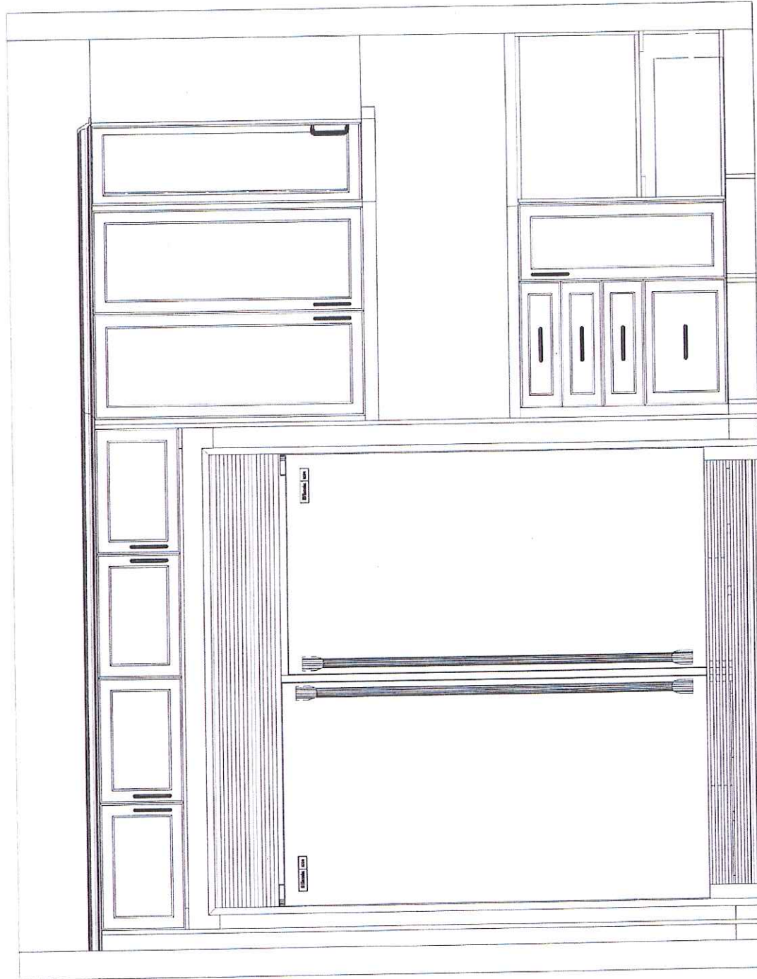
FRIDGE / FREEZER WALL ELEVATION
