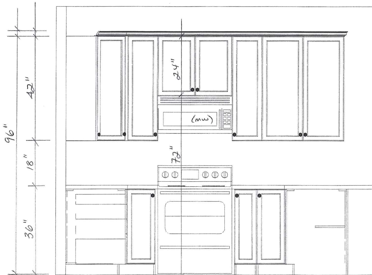
STOVE WALL ELEVATION
