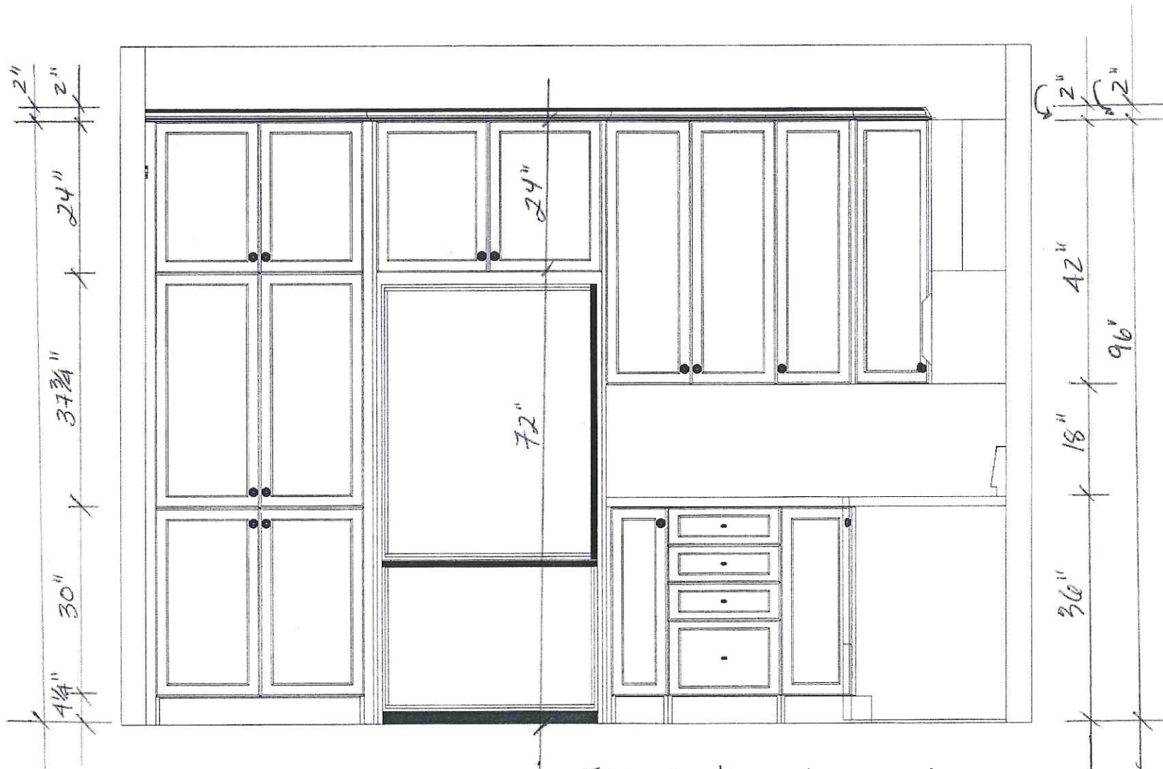
FRIDGE WALL ELEVATION
