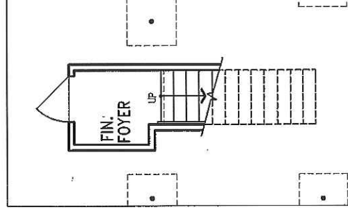
OPT. FIN. FOYER FOR OPEN STAIR
