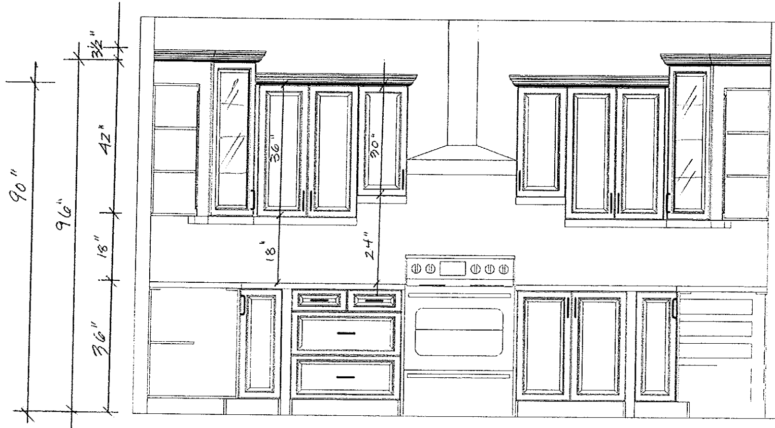
SPVE WALL ELEVATION
