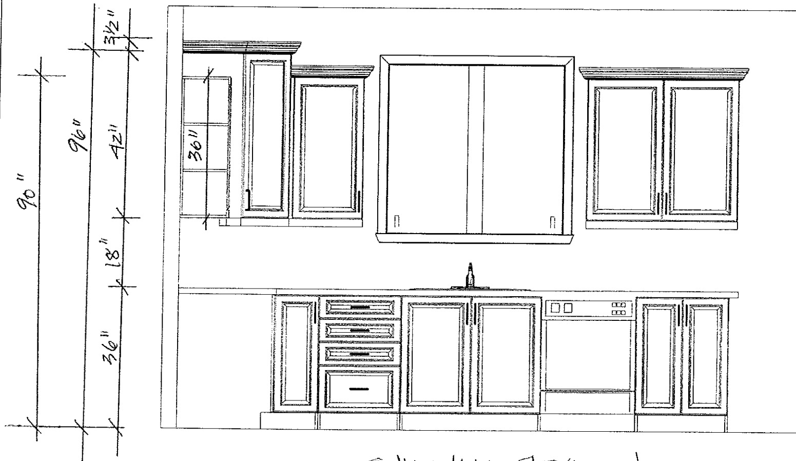
SINK WALL ELEVATION
