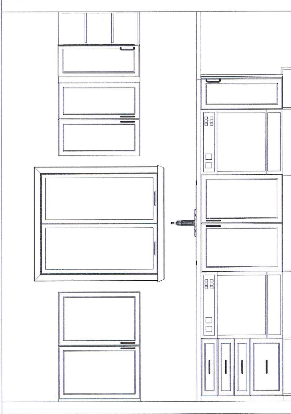
SINK WALL ELEVATION
