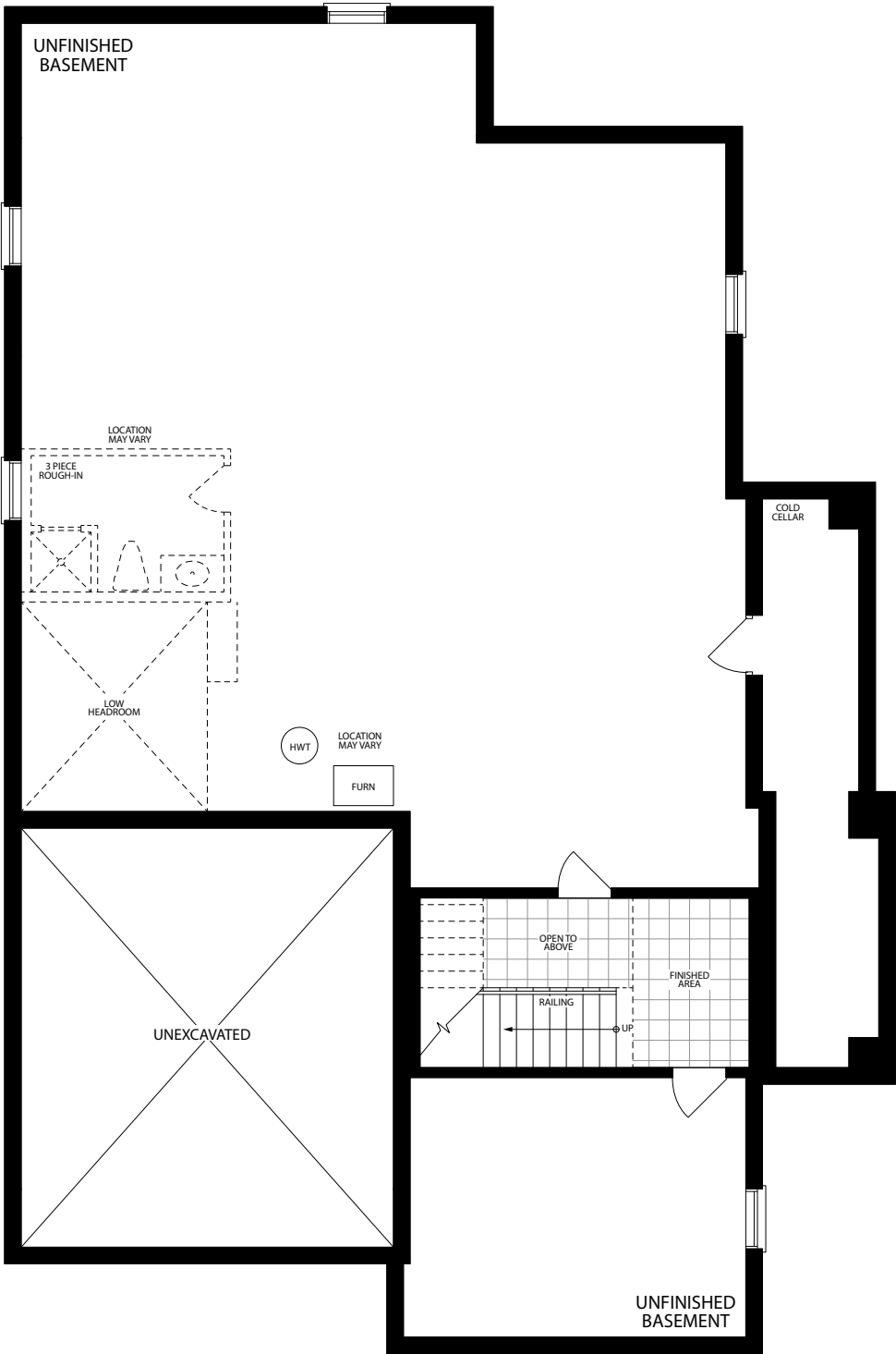
BASEMENT FLOOR ELEVATION C
