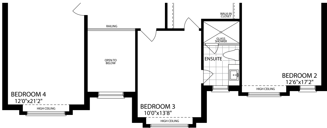
SECOND FLOOR ELEVATION C
