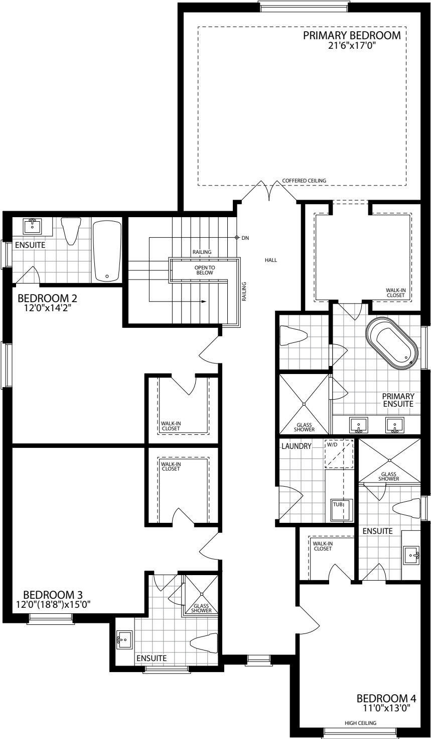
SECOND FLOOR ELEVATION C
