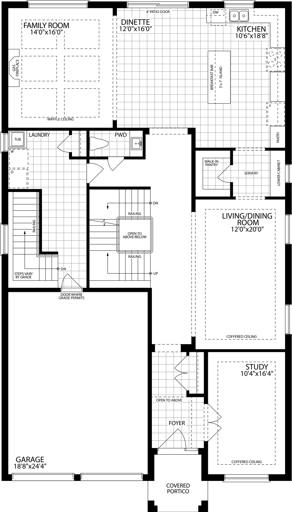
GROUND FLOOR ELEVATION B
