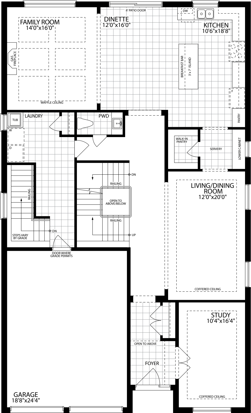
GROUND FLOOR ELEVATION A
