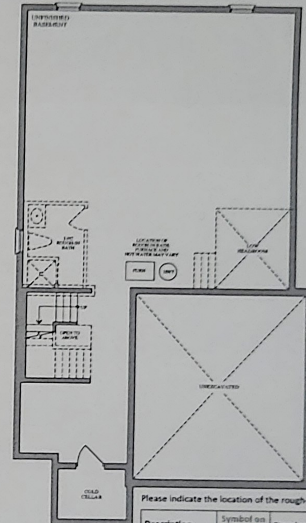
BASEMENT ELEVATION A & B
